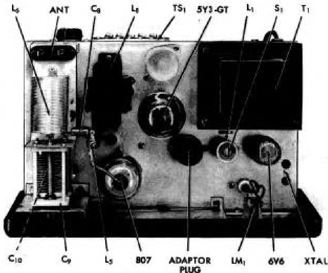
Figure 3. Top View of Chassis.
