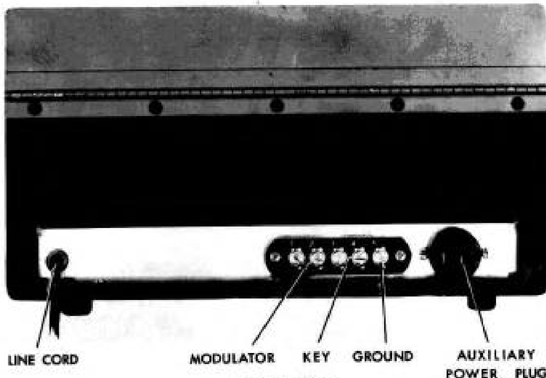
Figure 2. Rear View.
